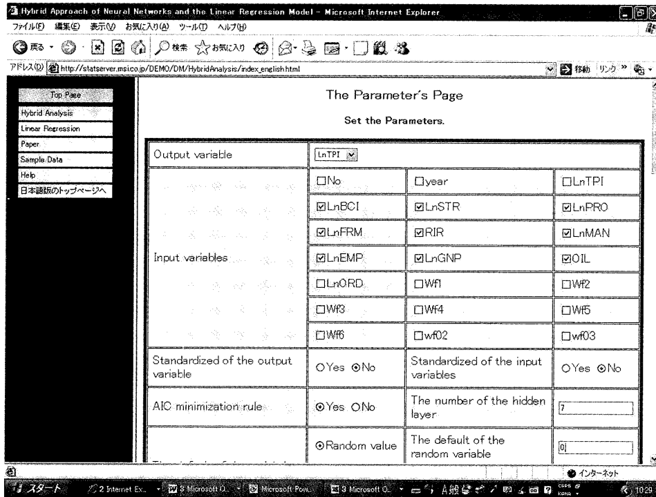
Figure 1. Parameter's Page (1).
