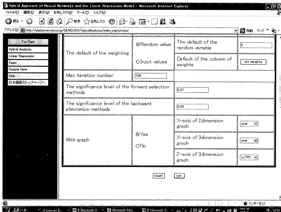
Figure 2. Parameter's Page (2).
