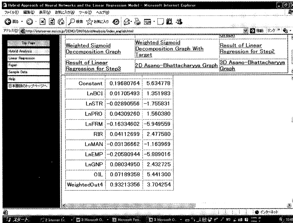
Figure 7. Result of Linear Regression for Step2. ( p = 9 , q = 6 , and q' = 1 )
